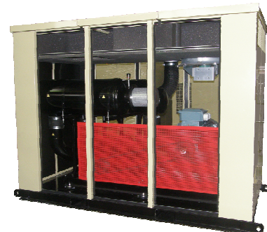
VP package for pneumatic conveying of fly ash in cement works
