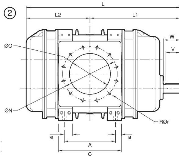
Vertical Configuration
