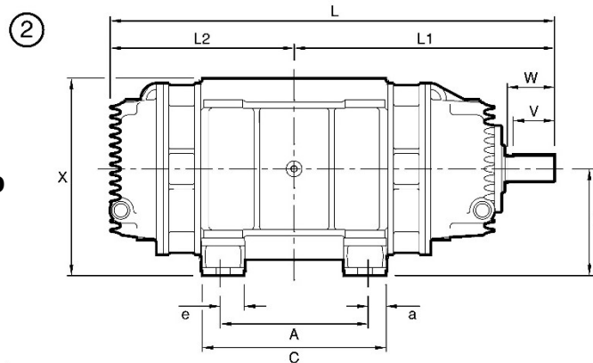
Horizontal Configuration
